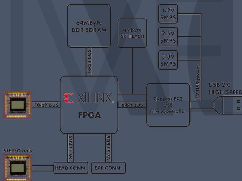
Figure 1: Camera structure block scheme
