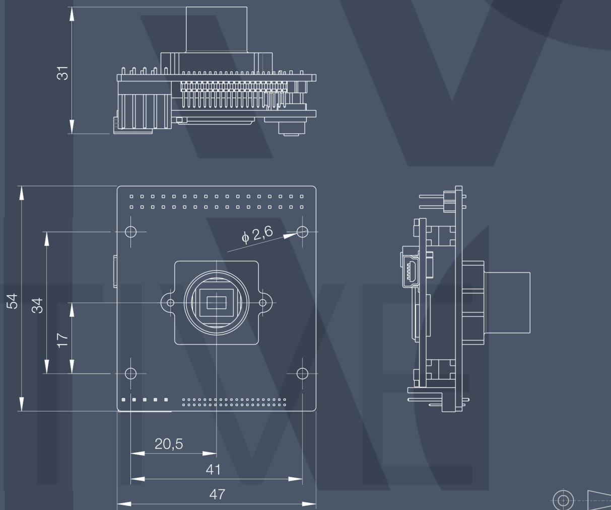
Figure 4: Cameleon Baseboard in OEM version and M12 lens holder
